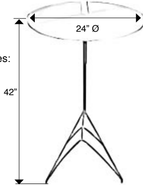
Tre3 STACKING BAR TABLE ITEM# 6TR24B Dimensions: 24"Ø x 42"h Net weight: 22.5 lb.
